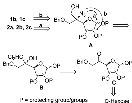
Scheme 1. Retrosynthesis of 1 and 2
