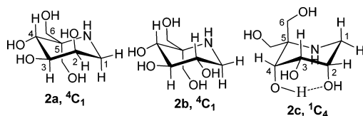
Figure 5. Conformations of 2a, 2b and 2c.
