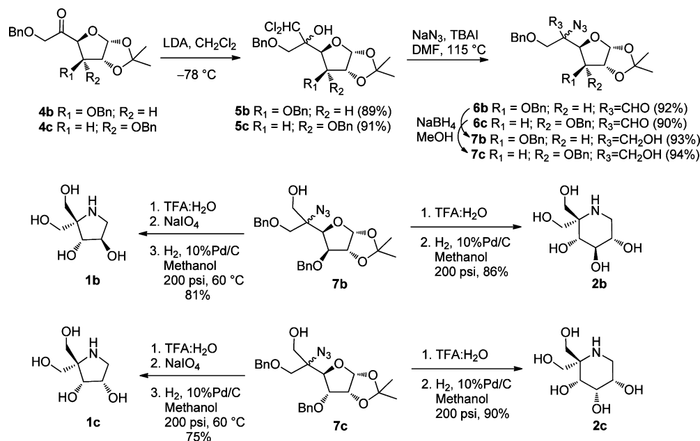
Scheme 3. Synthesis of Iminosugars 1b, 1c, 2b, 2c
