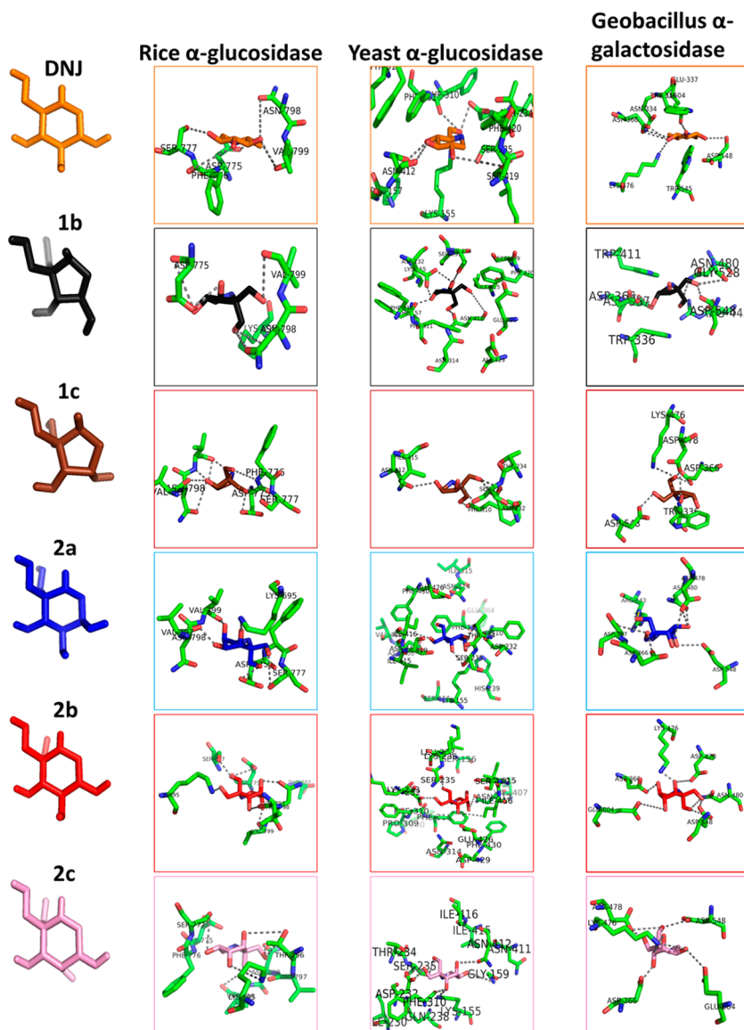
Figure 6. Binding of ligands DNJ, 2a, 2b, 2c, 1b, and 1c with active pocket of rice \alpha -glucosidase, yeast \alpha -glucosidase and Geobacillus \alpha -galactosidase.
