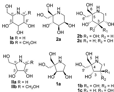
Figure 1. Piperidine and pyrrolidine iminosugars.
